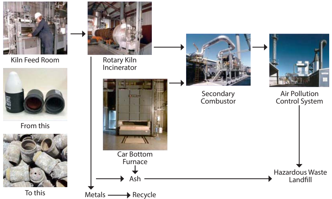
Incineration Process
